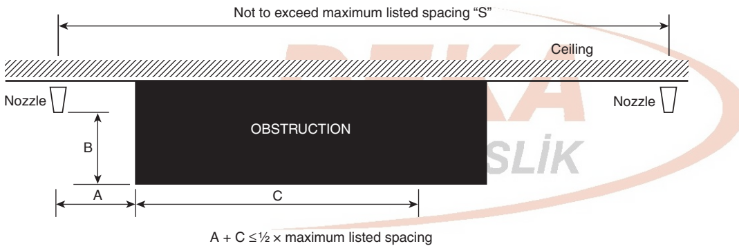
FIGURE A.7.2.5(c) Dimensions Governing the Position of Nozzles on Either Side of a Continuous Obstruction.
