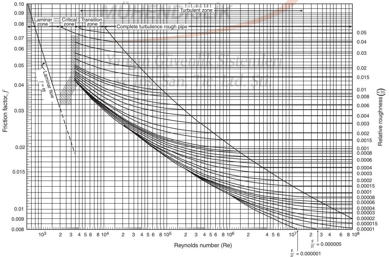
FIGURE 9.2.2 Moody Diagram.
