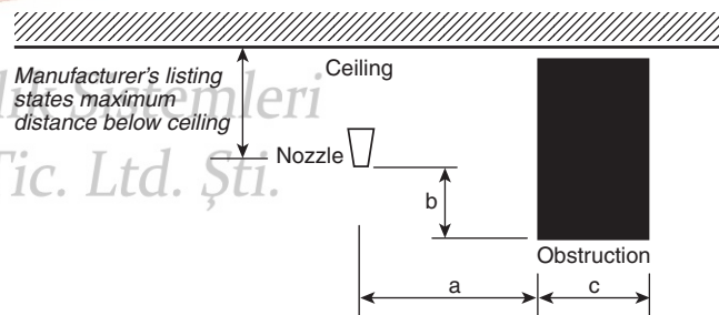
FIGURE A.7.2.5(a) Dimensions to Be Considered for Locating Nozzles Relative to Beam, Duct, or Other Continuous Obstruction.
