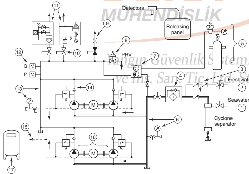
FIGURE A.11.1.6(e) Schematic Diagram of a Pump-Driven Water Mist System. [Typical]
