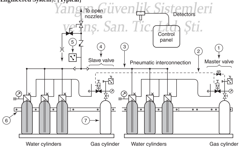
FIGURE A.11.1.6(a) Schematic Representation of a High Pressure, Gas-Driven System with Stored Water (Pre-Engineered System). [Typical]
