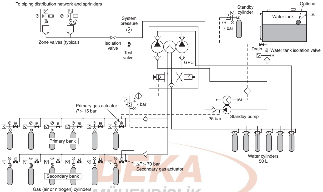
FIGURE A.11.1.6(i) Gas Pump for Light Hazard Applications. [Typical]
