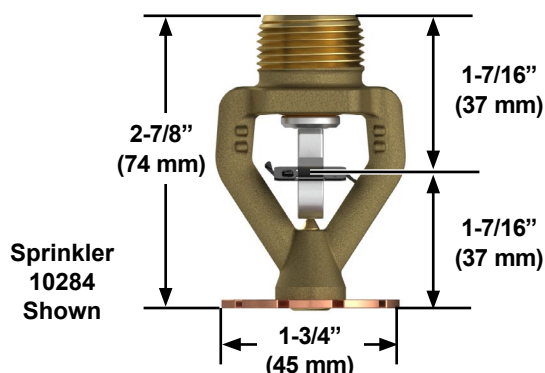
Figure 2: ESFR Pendent Sprinkler VK500 Dimensions
